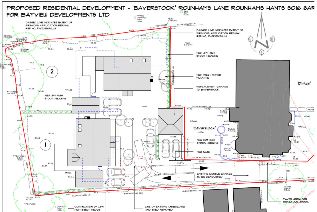
Figure 2 – Site plan
